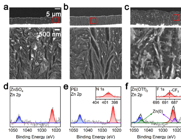
Fig. 5 HIM images and XPS spectra. (top) HIM images and (bottom) magnified images of the region outlined in red in the top images of the passivation layer formed in the (a) 1 M ZnSO 4 , (b) 1 M ZnSO 4 + 100 ppm PEI, and (c) 1 M Zn(OTf) 2 electrolytes after the first cycle at a (charging/discharging) current density of 76 mA cm -2 in a model zinc air battery. XPS Zn 2p, N 1s, and F 1s spectra of the surface of the passivation layer after the first cycle: (d) 1 M ZnSO 4 , (e) 1 M ZnSO 4 + 100 ppm PEI, and (f) 1 M Zn(OTf) 2 .
