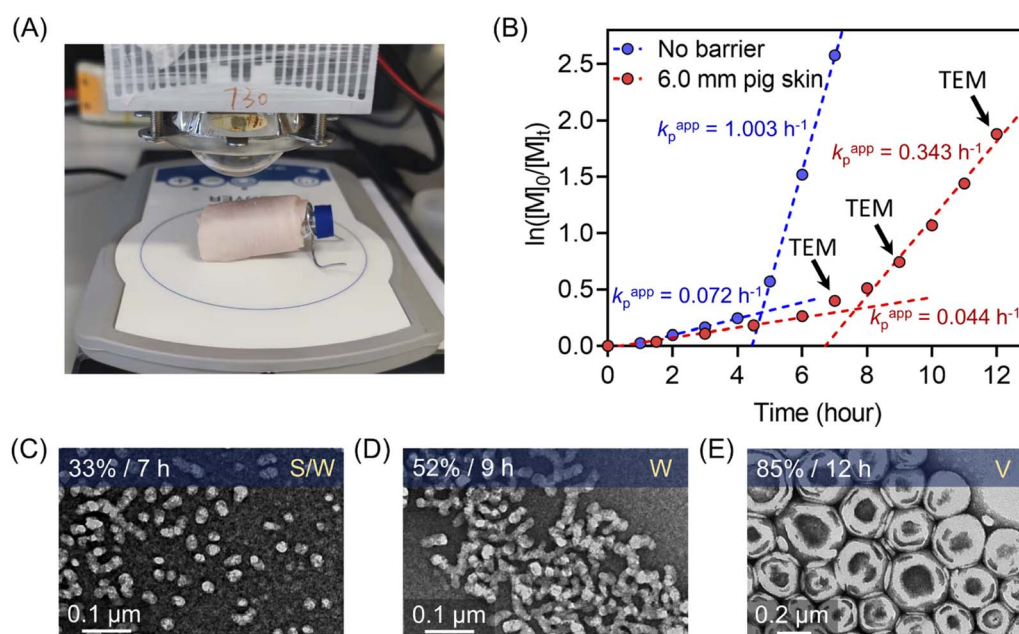
Fig. 7 (A) Experimental setup of photo-RAFT dispersion polymerization under the NIR light ( \lambda_{max} = 730 nm; 60 mW cm^{-2} ) irradiation passing through 6.0 mm pig skin. (B) Comparison of dispersion photo polymerization kinetics between without barrier and through 6.0 mm pig skin. (C–E) Evolution of morphologies of polymeric nanoparticles synthesized through 6.0 mm pig skin indicated by corresponding TEM images at different time points ( t = 7, 9, and 12 hours).
