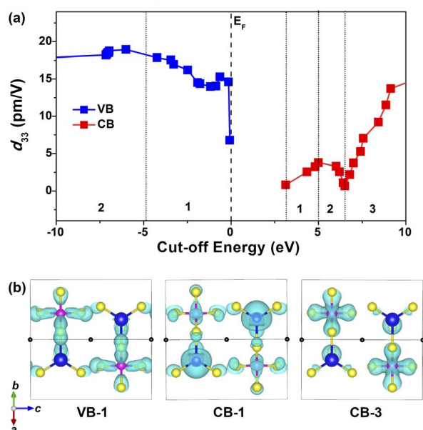
Fig. 7 Theoretical analysis of the SHG source for SrCdSi 4 : (a) variation of cut-off energy (eV) versus the largest static d_{33} ; (b) charge-density-cuts in the selections (VB-1, CB-1, CB-3) of major contribution. Black atoms: Sr; blue atoms: Cd; pink atoms: Si; yellow atoms: S.
