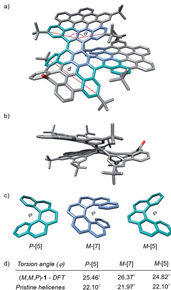
Fig. 2 (a) DFT optimized geometry of ( M,M,P )- 1 (CAM-B3LYP/6-31G(d,p), gas phase; lateral ^t\text{Bu} groups removed to reduce computational time); (b) side view; (c) [ n ]helicene structures extracted from the optimized geometry; (d) values of the measured torsion angles from the DFT optimized ( M,M,P )- 1 and XRD structures of pristine helicenes.
