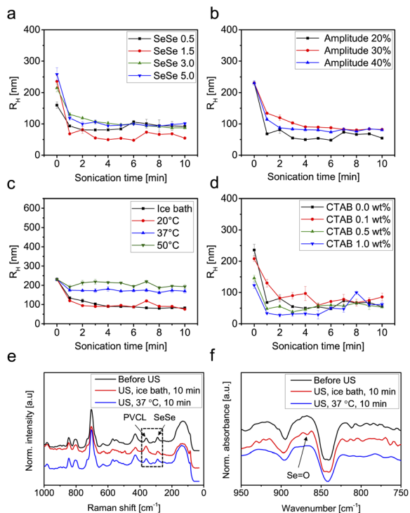
Fig. 3 R_H over the course of sonication and after dialysis of (a) \text{Se}_\mu\text{G} with 0.5, 1.5, 3.0, and 5.0 mol% diselenide contents, (b) Se 1.5 mol% with 20, 30, and 40% amplitude, (c) Se 1.5 mol% at different temperatures, and (d) Se 1.5 mol% synthesized with 0, 0.1, 0.5, and 1.0 wt% of CTAB. Sonication experiments of (a), (b), and (d) were performed in an ice bath, and (c), and (d) were performed at 30% amplitude. Power intensity for 30% amplitude was I_p = 1.82 \text{ W cm}^{-2} . (e) Raman and (f) IR spectra of Se1.5 before and after 10 min ultrasonication in an ice bath at 37 °C.
