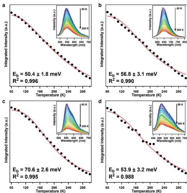
Fig. 3 Integrated photoluminescence intensity as a function of temperature from 80 to 300 K of (a) PTz-TPB-COF, (b) PTz-BTA-COF, (c) PTz-Py-COF, and (d) OPTz-BTA-COF. The red curves represent the fitting by using the Arrhenius equation. The inset is the temperature-dependent photoluminescence spectra for each COF.
