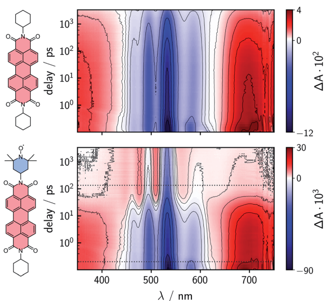
Fig. 3 Contour plots of the fsTA data of PDI 0sg (top) and PDI 0sg -TEMPO (bottom) recorded at room temperature in toluene. The red and blue color coding represents positive and negative signals, respectively. The horizontal black dotted lines in the contour plot of PDI 0sg -TEMPO indicate the time delays corresponding to the spectra in Fig. 4.
