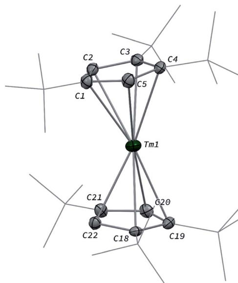
Fig. 2 Molecular structure of one of the two independent molecules of 1 in the solid state with thermal ellipsoids at the 40% probability level (except for the 'Bu groups depicted in wireframe). Only one disordered position for the 'Bu groups has been depicted and H atoms have been omitted for clarity. Selected bond distances (Å): Tm1–C1 2.712(4), Tm1–C2 2.676(4), Tm1–C3 2.681(4), Tm1–C4 2.664(4), Tm1–C5 2.670(4), Tm1–C18 2.673(4), Tm1–C19 2.677(4), Tm1–C20 2.686(4), Tm1–C21 2.703(4), Tm1–C22 2.658(4).
