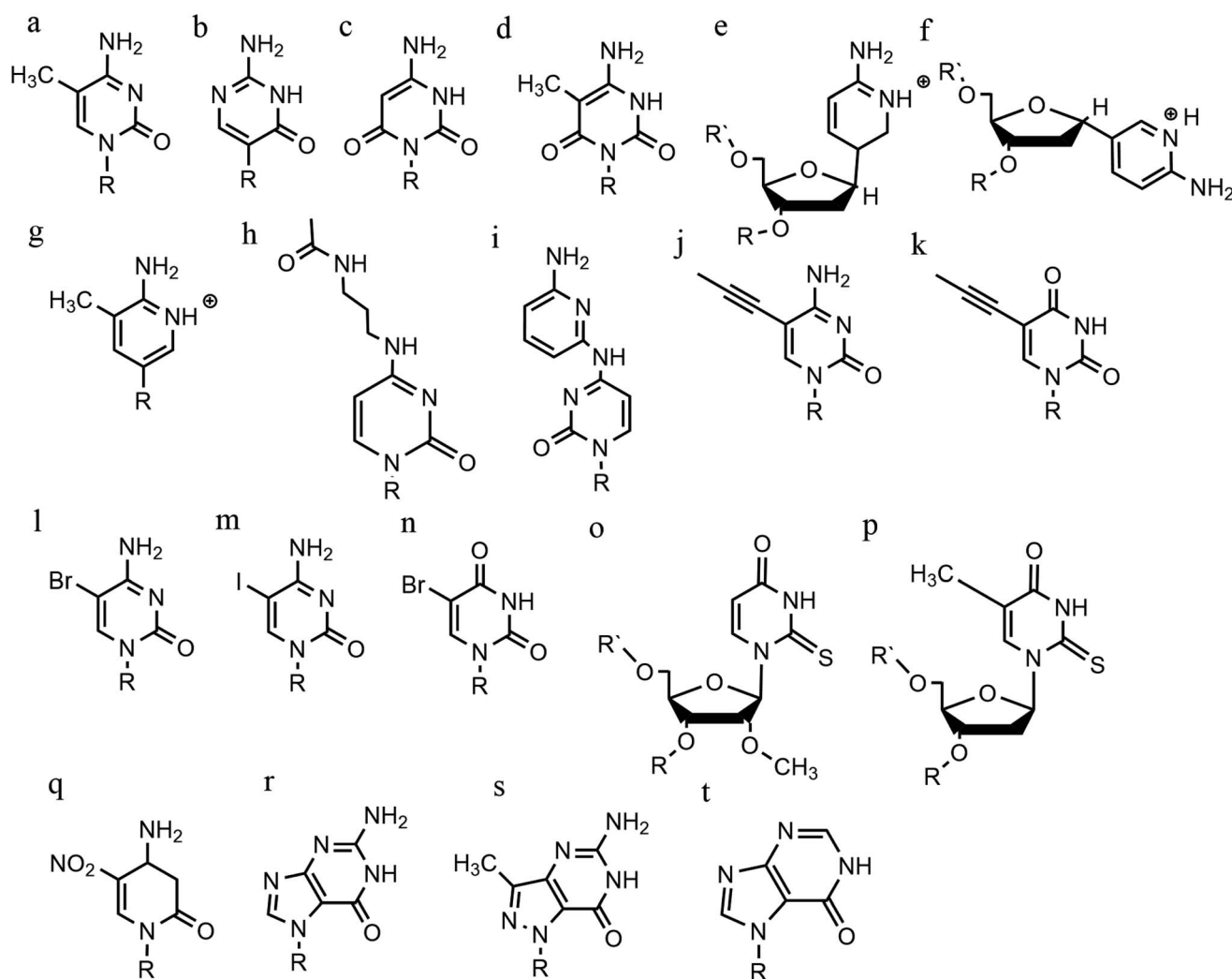
Fig. 9 Base modifications in parallel triplexes. (a) 5-Methyl-cytosine, (b) 2'-O-methyl-pseudocytidine, (c) 6-oxo-cytosine, (d) 5-methyl-6-oxo-cytosine, (e) \alpha -AP, (f) \beta -AP, (g) 2'-aminoethoxy-thymine, (h) N^4 -3-acetamidopropyl-cytosine, (i) N^4 -6-aminopyridinyl-cytosine, (j) 5-propynyl-cytosine, (k) 5-propynyl-uracil, (l) 5-bromo-cytosine, (m) 5-iodo-cytosine, (n) 5-bromo-uridine, (o) 2'-O-methyl-2-thio-uridine, (p) 2-thio-thymidine, (q) 6-amino-5-nitropyridin-2-one, (r) N7-glycosilated-guanine, (s) P1-guanine, (t) inosine.
