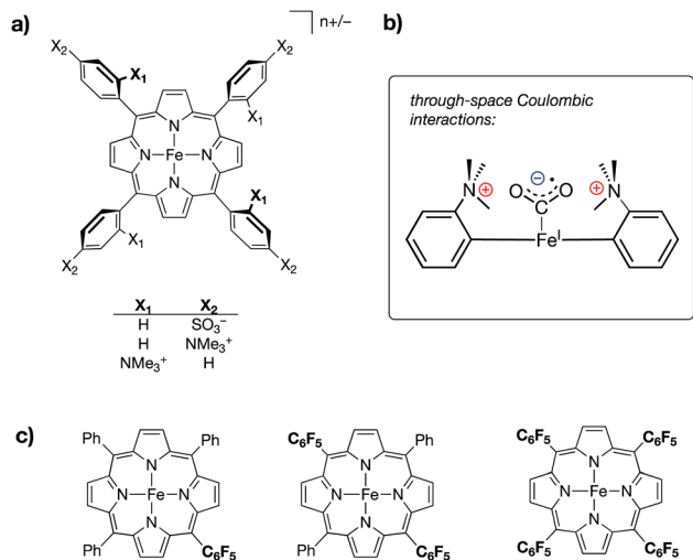
Fig. 9 (a) Iron tetraphenylporphyrin-based CO 2 reduction electrocatalysts containing either cationic (–NMe 3 + ) or anionic (–SO 3 - ) substituents at different positions on the porphyrin phenyl rings; 60 (b) schematic of a proposed through-space coulombic interaction between cationic ammonium groups on the tetraphenylporphyrin ligand and a bound CO 2 - molecule; and (c) a series of iron tetraphenylporphyrin complexes in which inductive effects were systematically modulated through incorporation of pentafluorophenyl substituents.
