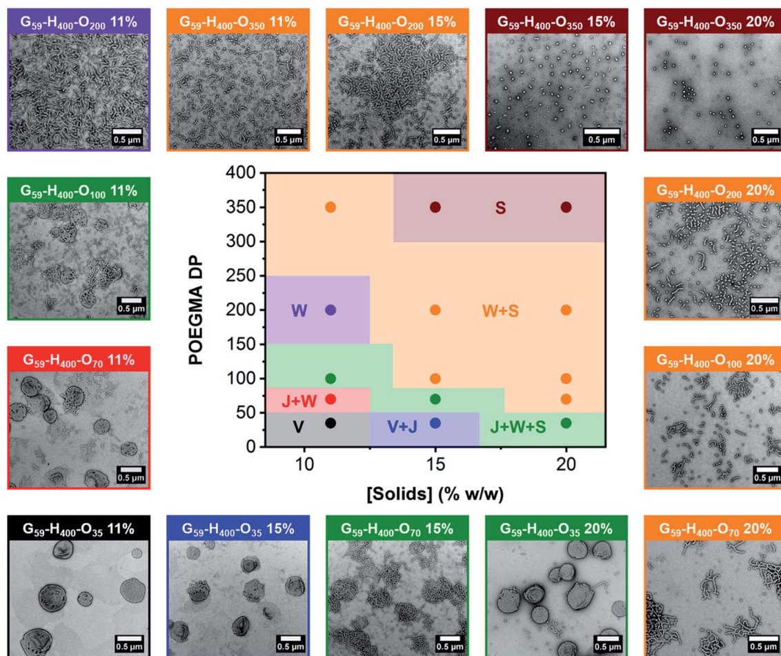
Fig. 3 Pseudo-phase diagram constructed for G_{59} - H_{400} - O_x triblock copolymer nano-objects ( x = 35 – 350 ) prepared via RAFT-mediated aqueous PIDA by systematically varying the total solids content and target POEGMA DP. Representative TEM images obtained using a 0.75% w/w uranyl formate staining solution are shown for each formulation. Each frame color corresponds to a different nano-object morphology (S = spherical micelles; W = worms; J = jellyfish and V = vesicles).
