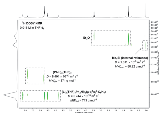
Fig. 6 ^1\text{H} DOSY NMR spectrum showing the dissociation of 5 in THF- d_8 .
