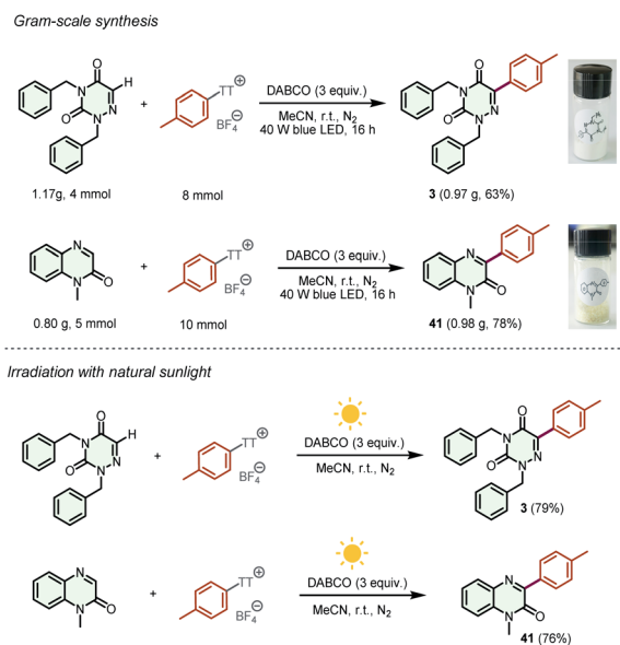
Scheme 5 Synthetic applications.
