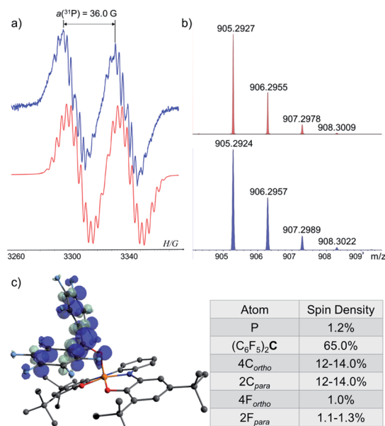
Fig. 7 (a) EPR spectra of [1\text{-OC(C}_6\text{F}_5)_2]^\bullet (blue) and its simulation (red); (b) MS of the reduced [1\text{-OC(C}_6\text{F}_5)_2]^\bullet ( 905.2927 (M) ^- ) (red) and its simulation (blue); (c) DFT calculated Mulliken atomic spin densities in [1\text{-OC(C}_6\text{F}_5)_2]^\bullet .
