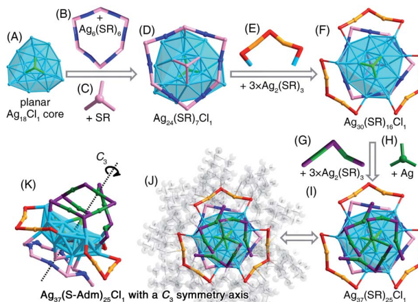
Fig. 7 Structural anatomy of [\text{Ag}_{37}(\text{S-Adm})_{25}\text{Cl}_1]^+ . (A) The planar \text{Ag}_{18}\text{Cl}_1 core + (B) the \text{Ag}_6(\text{SR})_6 ring-like motif + (C) the capping SR = (D) The \text{Ag}_{24}(\text{SR})_7\text{Cl}_1 structure. (E) Three \text{Ag}_2(\text{SR})_3 dimeric motifs. (F) The \text{Ag}_{30}(\text{SR})_{16}\text{Cl}_1 structure. (G) Three \text{Ag}_2(\text{SR})_3 dimeric motifs. (H) The bridging Ag. (I) The \text{Ag}_{37}(\text{SR})_{25}\text{Cl}_1 framework. (J) and (K) The overall structure of [\text{Ag}_{37}(\text{S-Adm})_{25}\text{Cl}_1]^+ exhibits a C_3 symmetry axis. Color legends: light blue/blue/orange/green sphere, Ag; pink/orange/purple sphere, S; light green sphere, Cl; grey sphere, C; light grey sphere, H.
