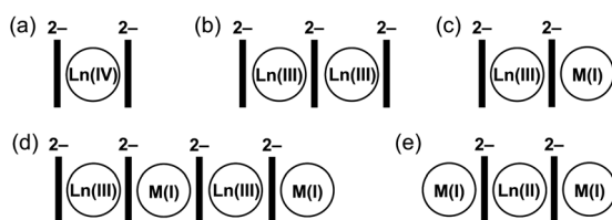
Scheme 1 Depiction of crystallographically characterized homoleptic Ln complexes with the COT 2- ligand.
