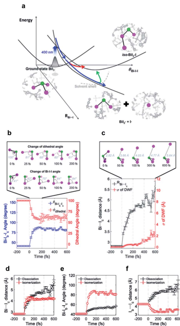
Fig. 3 (a) Schematic representation of the photodynamics of \text{BiI}_3 in acetonitrile. (b) Changes of the \text{Bi-I}_b - \text{I}_c angle and \text{I}_a - \text{Bi-I}_b - \text{I}_c dihedral angle during the roaming-mediated isomerization determined from structural analysis on the fs-TRXL data for \text{BiI}_3 in acetonitrile. (c) Changes of the \text{Bi}\cdots\text{I}_c distance and the root-mean-squared displacement ( \sigma ) associated with the pair distances containing \text{I}_c . Insets in (b) and (c) show transient structures at representative time delays. (d-f) Comparison of the structural motions for the dissociation and roaming-mediated isomerization channels through (d) \text{Bi}\cdots\text{I}_c distance, (e) \text{Bi-I}_b - \text{I}_c angle, and (f) \text{I}_b\cdots\text{I}_c distance. Reproduced from ref. 65 with the permission of Springer Nature, copyright 2021.
