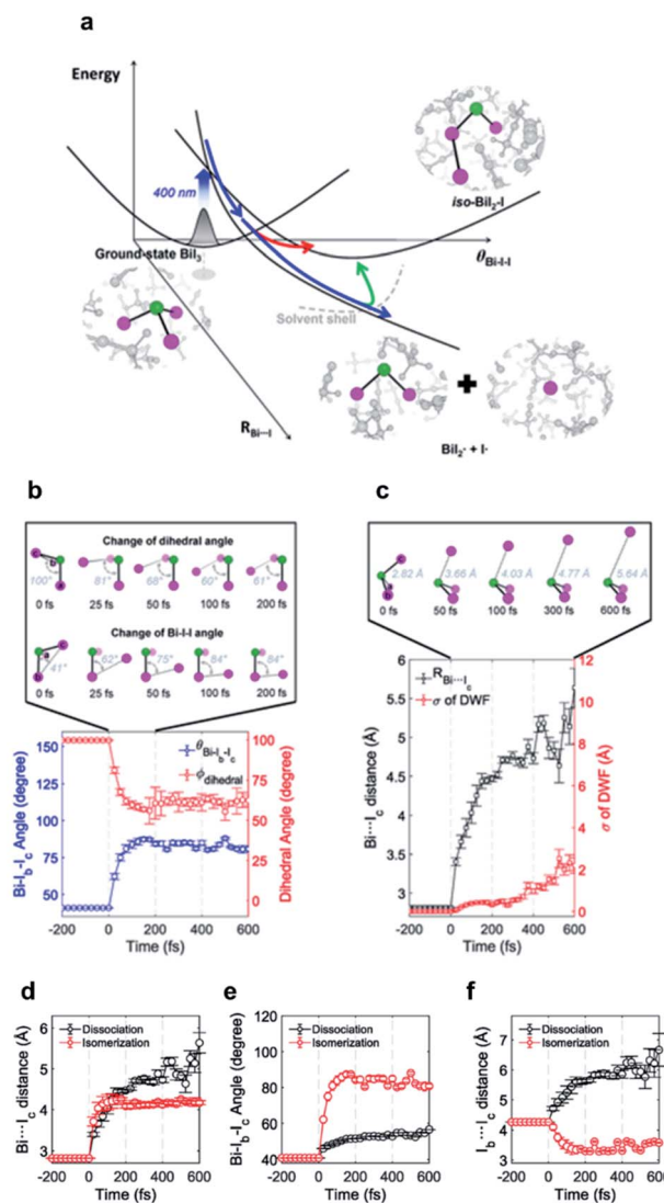
Fig. 3 (a) Schematic representation of the photodynamics of \text{BiI}_3 in acetonitrile. (b) Changes of the \text{Bi-I}_b\text{-I}_c angle and \text{I}_a\text{-I}_b\text{-I}_c dihedral angle during the roaming-mediated isomerization determined from structural analysis on the fs-TRXL data for \text{BiI}_3 in acetonitrile. (c) Changes of the \text{Bi}\cdots\text{I}_c distance and the root-mean-squared displacement ( \sigma ) associated with the pair distances containing \text{I}_c . Insets in (b) and (c) show transient structures at representative time delays. (d–f) Comparison of the structural motions for the dissociation and roaming-mediated isomerization channels through (d) \text{Bi}\cdots\text{I}_c distance, (e) \text{Bi-I}_b\text{-I}_c angle, and (f) \text{I}_b\cdots\text{I}_c distance. Reproduced from ref. 65 with the permission of Springer Nature, copyright 2021.
