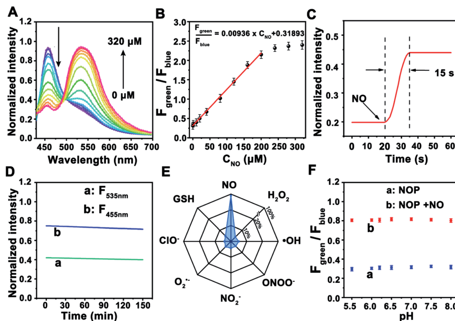
Fig. 2 (A) TPF emission spectra of the NOP with the addition of different concentrations of NO ( 0, 0.1, 10.0, 20.0, 40.0, 80.0, 120.0, 160.0, 200.0, 240.0, 280.0, and 320.0\ \mu\text{M} ) in cell lysates. (B) Calibration curve between F_{\text{green}}/F_{\text{blue}} and various concentrations of NO ( n = 5 , S. D.). (C) Response time of the NOP with the addition of NO ( 50\ \mu\text{M} ). (D) Photostability of the NOP at 455\text{ nm} ( F_{455\text{nm}} ) and 535\text{ nm} ( F_{535\text{nm}} ) after the NOP was exposed to a Xe lamp ( 90\text{ W} ). (E) Selectivity tests of the NOP toward common RNS ( 100\ \mu\text{M} ) and ROS ( 100\ \mu\text{M} ). (F) F_{\text{green}}/F_{\text{blue}} values of the NOP at pH 5.0\text{--}8.0 in the absence (a) and in the presence (b) of NO ( 50\ \mu\text{M} ) ( n = 5 , S. D.).
