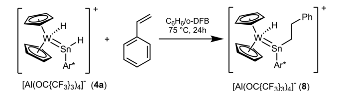
Scheme 7 Insertion of styrene into a Sn–H bond.
