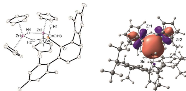
Fig. 4 ORTEP and NLMO exhibiting the three centre two electron bond of cation [(\text{Cp}_2\text{ZrH})_2\text{HSnHAr}^*]^+ of 10 . Thermal ellipsoids are shown at 50% probability level. Hydrogen atoms except the Zr–H and Sn–H units, methyl groups and the anion of 10 have been omitted. Selected interatomic distances [Å] and angles ^\circ : Zr1–Sn 3.0185(2), Zr2–Sn 3.0325(2), Zr1–Zr2 3.577(2), Zr1–Cp 2.4845(14) – 2.5328(15), Zr2–Cp 2.4760(14) – 2.5162(15), Sn–C1 2.1678(12), Sn–H1 1.57(3), Sn–H2 2.07(3), Sn–H3 1.98(3), Zr1–H2 1.84(3), Zr1–H4 2.00(2), Zr2–H3 1.89(3), Zr2–H4 1.97(2), Zr1–Sn–Zr2 72.5(1), C1–Sn–H1 95.8(10), H2–Sn–H3 144.7(11), H2–Zr1–H4 121.6(11), H3–Zr2–H4 118.3(10).
