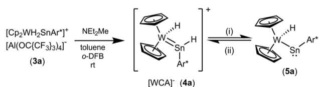
Scheme 4 (i) ^{\text{Me}}\text{NHC} , toluene/ \text{C}_6\text{H}_4\text{F}_2 , 70^\circ\text{C} , 3 d, -\text{[}^{\text{Me}}\text{NHC-H]Al(OC(CF}_3)_3)_4^- ; (ii) \text{H(Et}_2\text{O)}_2[\text{BARF}] toluene/ o -DFB. \{\text{B(3,5-(CF}_3)_2\text{C}_6\text{H}_3)_4\}^- = [\text{BARF}]^- .
