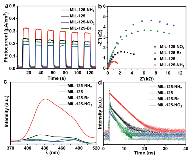
Fig. 3 (a) Photocurrent responses, (b) EIS Nyquist plots, (c) photoluminescence (PL) spectra (excited at 250 nm), and (d) time resolved PL spectra for MIL-125 and MIL-125-X ( X = \text{NH}_2, \text{NO}_2, \text{Br} ) in MeCN.
