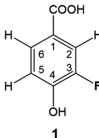
Fig. 1 3-Fluoro-4-hydroxybenzoic acid, 1 .
