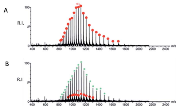
Fig. 9 (A) Representative ESI-MS spectrum of a solution containing 10 \mu M SARS-CoV-2 M pro in water/acetonitrile (50 : 50) added with 0.1% formic acid. The spectrum was acquired in positive ion mode. (B) Representative ESI-MS spectrum of a mixture containing 10 \mu M SARS-CoV-2 M pro after incubation with QUB-00006-Int-07 (compound : protein ratio = 10 : 1) in water/acetonitrile (50 : 50) added with 0.1% formic acid. The spectrum was acquired in positive ion mode. The red dots correspond to the unmodified protein, and the green asterisks correspond to the modified protein.
