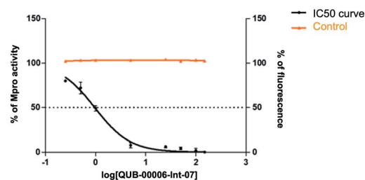
Fig. 8 Dose-response curves obtained by plotting the percentage of SARS-CoV-2 M pro residual activity as a function of increasing concentrations of QUB-00006-Int-07 (0–150 \mu M). [M pro ] = 20 nM, [PS1] = 5 \mu M, %DMSO = 3.75%. Experiments were performed in triplicate. A counter screening control experiment was performed by testing increasing concentrations of QUB-00006-Int-07 in the presence of 0.5 \mu M free fluorescein.
