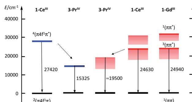
Fig. 6 Partial electronic diagram for 1-Ce, 3-Pr MeCN , and 1-Gd. Calculated levels in blue, experimental 0-phonon levels in red or rose when estimated from the onset of the emission band. Energies of the transitions in \text{cm}^{-1} .
