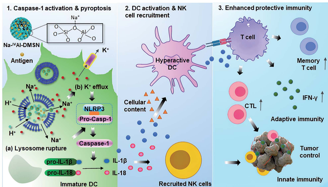
Scheme 1 Proposed mechanisms for \text{Na-IVAl-DMSN} induced DC pyroptosis and hyperactivation for enhanced innate immunity and adaptive immunity for tumor prophylaxis.
