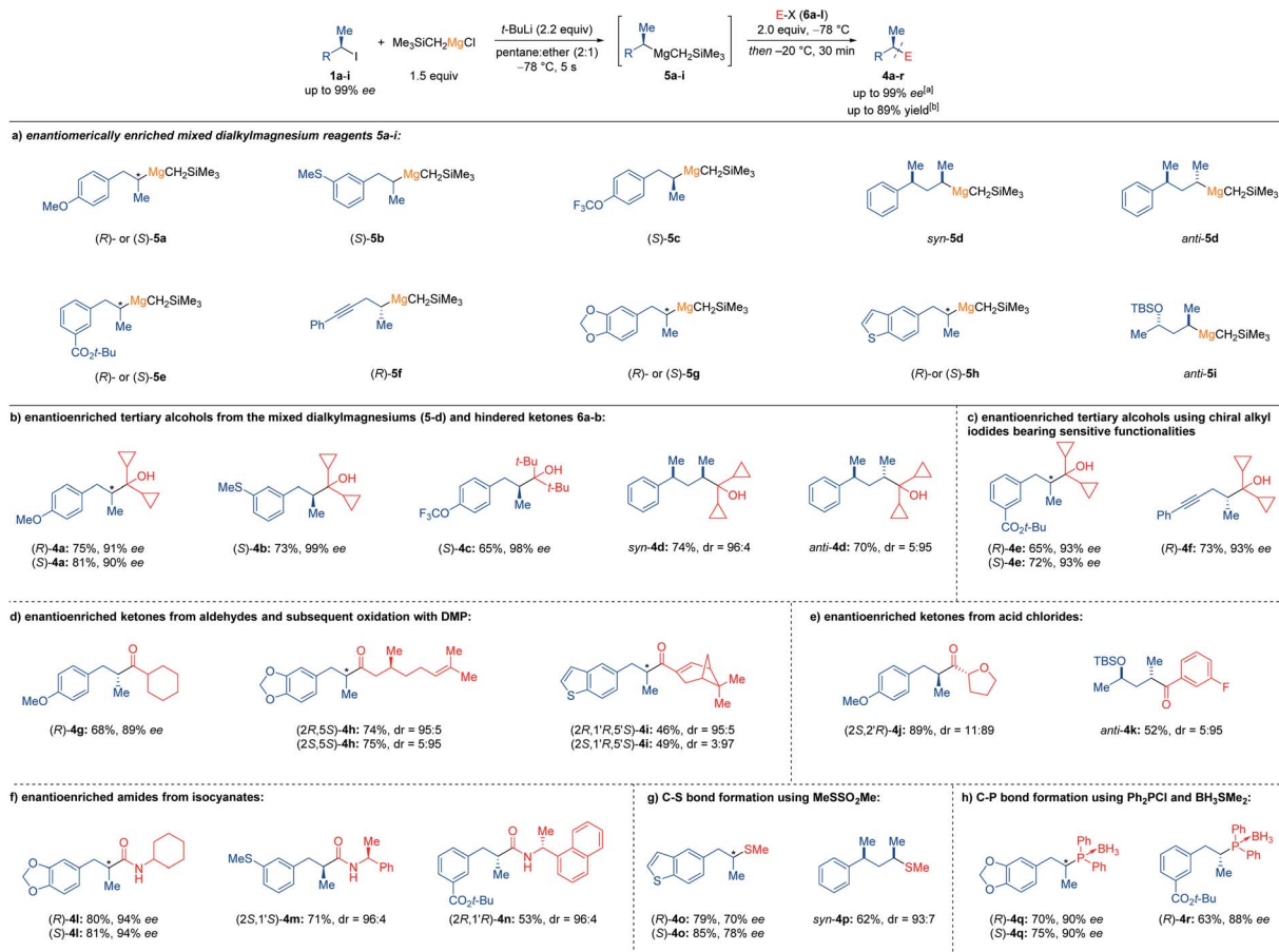
Scheme 2 Scope of optically enriched secondary alkylmagnesium reagents 5a-i and subsequent reactions with electrophiles ( 6a-l ). Enantio- and diastereomerically enriched secondary alkylmagnesium reagents 5a-i prepared by an I/Li-exchange in the presence of Me 3 SiCH 2 MgCl and their reactions with electrophiles ( 6a-l ) leading to the corresponding optically and diastereomerically enriched products 4a-r . a The enantiomeric excess (% ee) was determined by chiral HPLC-analysis. The diastereomeric ratio (dr; syn/anti ratio) was determined by 1 H-NMR spectroscopy and GC-analysis. b Yield refers to isolated analytically pure compounds.
