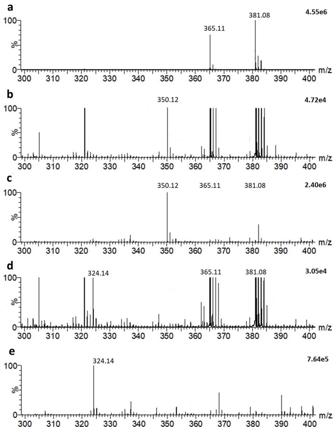
Fig. 4 (a) LAP-MALDI mass spectrum of bovine milk ( m/z 300–400). Sodiated lactose [M + \text{Na}]^+ is detected at m/z 365.11 and potassiated lactose [M + \text{K}]^+ at m/z 381.08. (b) LAP-MALDI mass spectrum of ampicillin ( m/z 350.12; [M + H]^+ ), spiked into milk at a concentration of 50 \mu\text{g mL}^{-1} . (c) LAP-MALDI mass spectrum of ampicillin ( m/z 350.12; [M + H]^+ ) in water at a concentration of 50 \mu\text{g mL}^{-1} . (d) LAP-MALDI mass spectrum of decarboxylated hydrolysed ampicillin ( m/z 324.14; [M + H]^+ ), obtained after 120 min incubation of ampicillin in milk ( 50 \mu\text{g mL}^{-1} ) with 3–6 units of penicillinase. (e) LAP-MALDI mass spectrum of decarboxylated hydrolysed ampicillin ( m/z 324.14; [M + H]^+ ), obtained after 120 min incubation of ampicillin in water ( 50 \mu\text{g mL}^{-1} ) with 3–6 units of penicillinase.
