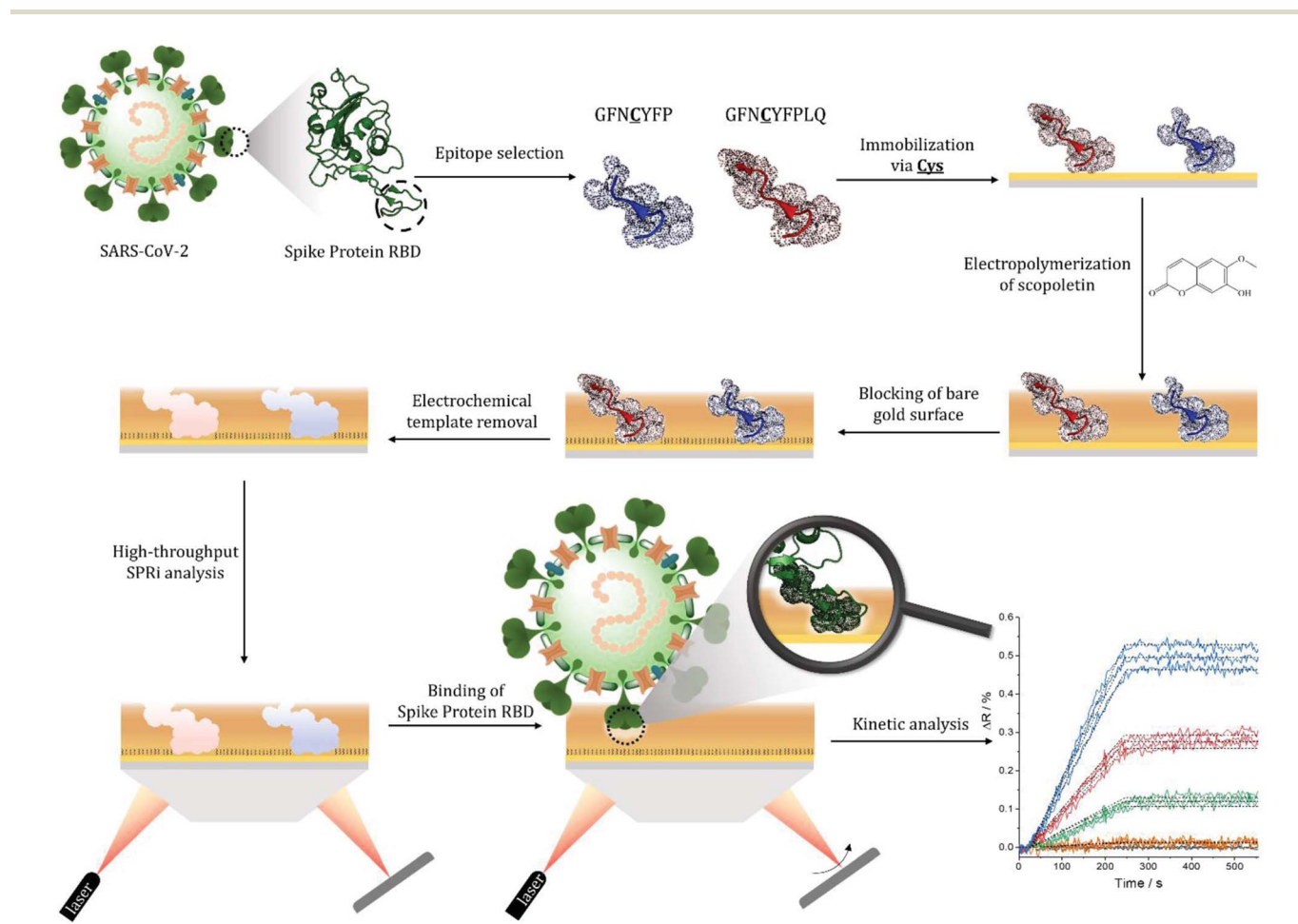
Scheme 1 Simplified workflow of the epitope-imprinted polymer synthesis and SPRi-based characterization. The selected nonapeptide epitope for the RBD of S protein (GFNCYFPLQ) bearing a central cysteine (and other relevant peptides, e.g. the heptapeptide GFNCYFP) are contact microspotted onto the surface of a gold SPRi chip resulting in ca. 500 \mu\text{m} diameter spots of the surface-immobilized peptides. This is followed by electropolymerization of scopoletin to form the epitope-imprinted polymer on the peptide spots, and blocking the contingently exposed gold surfaces by HS-TEG. The peptide templates are removed electrochemically by oxidative stripping to liberate the RBD selective cavities in the nanofilm. The kinetics of the target binding is then determined by SPRi for all spots of the microarray in label-free and multiplexed manner (the inset shows SPRi measurements for 3 identical spots, the colours denote different RBD concentrations).
