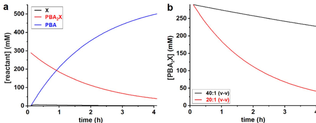
Fig. 2 Model curves for the concentrations of (a) PBA, free xylose and \text{PBA}_2\text{X} in the 20 : 1 dioxane system, and of (b) \text{PBA}_2\text{X} in the 40 : 1 and 20 : 1 dioxane–water systems.
