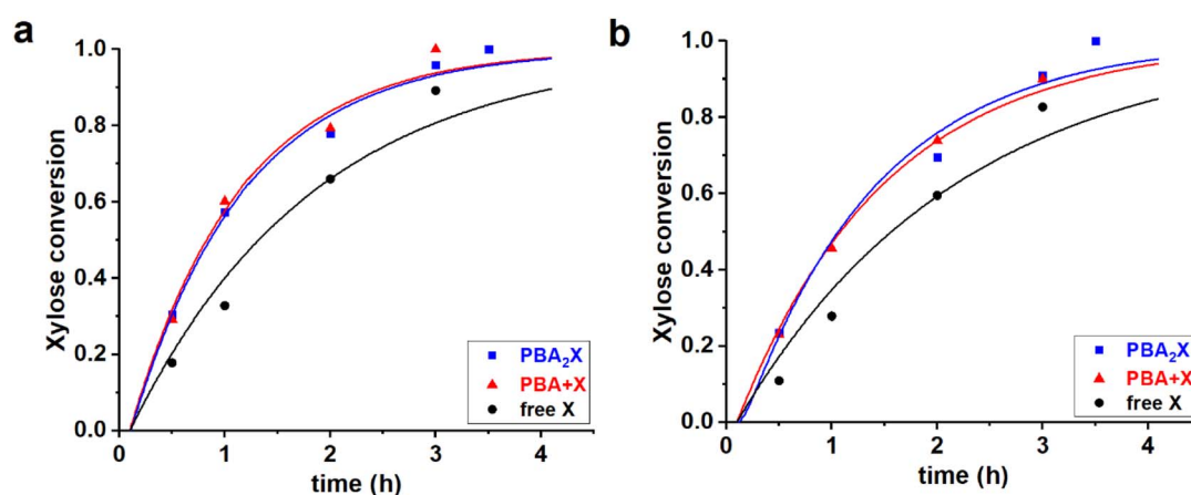
Fig. 3 Experimental data points (markers) and model curves (lines) for the xylose conversion for the reaction of dehydration of 94 mM of \text{PBA}_2\text{X} (blue), free xylose in presence of 194 mM PBA (red), and free xylose (black), performed at 180 °C in (a) 1 : 1 : 1 v/v/v of toluene–sulfolane–water (pH = 1) and (b) 1 : 1 : 1 v/v/v of MN–sulfolane–water (pH = 1) three-solvent systems. The raw data for toluene–sulfolane–water (a) have been reported before. 14
