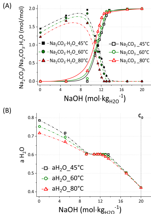
Fig. 8 PHREEQC simulation showing the molar ratio between the precipitated \text{Na}_2\text{CO}_3 and \text{Na}_2\text{CO}_3 \cdot \text{H}_2\text{O} (A) and the activity of water a_{\text{H}_2\text{O}} (B) at 45, 60 and 80^\circ\text{C} and increasing NaOH molalities, up to 20 m; the concentration C_0 (B) indicates the initial NaOH concentration considered for the samples here discussed.
