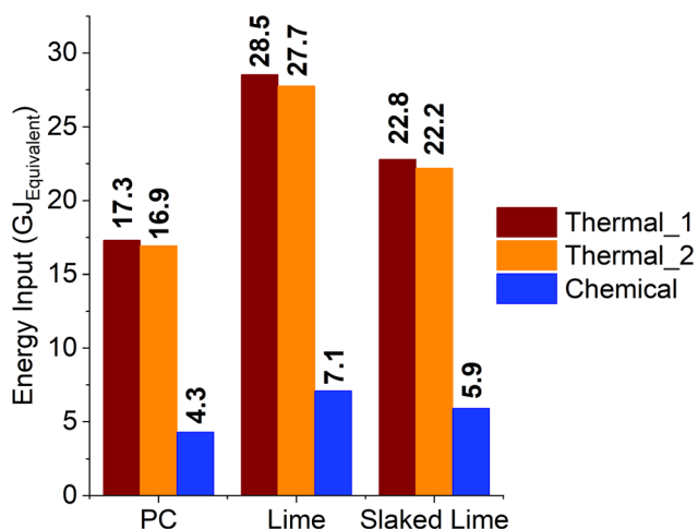
Fig. 11 Comparison of the energy consumption between the thermal and chemical approaches to the decarbonisation of CaCO 3 , referred to the cement, lime and slaked lime industries; the values only depend on the decarbonisation step, considering a PRK design for the thermal calcination in PC production, and PFRK one for lime and slaked lime.
