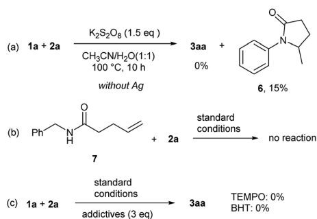
Scheme 5 Control experiments.
