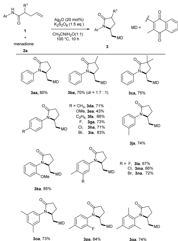
Scheme 2 Substrate scope of N -aryl-4-pentenamides ( 1 ). a,b a Reaction conditions: 1 (0.2 mmol), 2a (0.6 mmol), Ag 2 O (20 mol%), K 2 S 2 O 8 (1.5 equiv.) in CH 3 CN/H 2 O (1 : 1, 2.0 mL) for 10 h. b Isolated yields.
