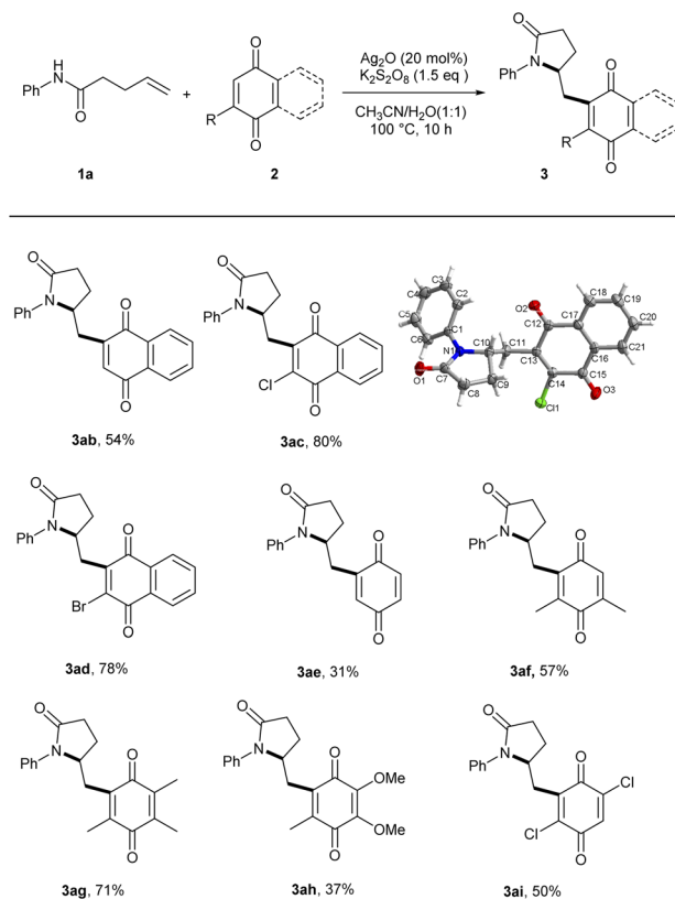
Scheme 3 Substrate scope of quinones ( 2 ). a,b a Reaction conditions: 1a (0.2 mmol), 2 (0.6 mmol), Ag 2 O (20 mol%), K 2 S 2 O 8 (1.5 equiv.) in CH 3 CN/H 2 O (1 : 1, 2.0 mL) for 10 h. b Isolated yields.
