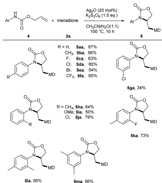
Scheme 4 Substrate scope of N -aryl allyl carbamates ( 4 ). a,b Reaction conditions: 4 (0.2 mmol), 2a (0.6 mmol), \text{Ag}_2\text{O} (20 mol%), \text{K}_2\text{S}_2\text{O}_8 (1.5 equiv.) in \text{CH}_3\text{CN}/\text{H}_2\text{O} (1 : 1, 2.0 mL) for 10 h. b Isolated yields.
