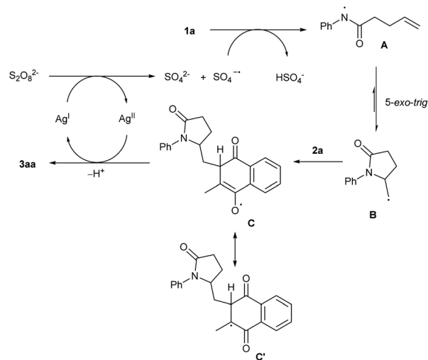
Scheme 6 Proposed mechanism.
