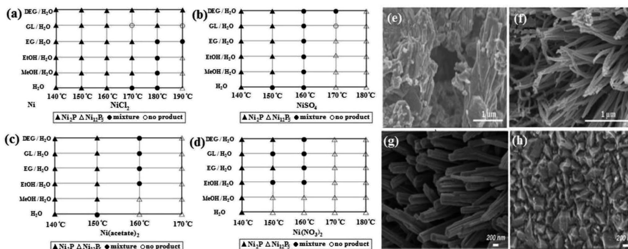
Fig. 4 Synthesis of nickel phosphides via the solvothermal method with different nickel precursors: (a) \text{NiCl}_2 \cdot 6\text{H}_2\text{O} , (b) \text{NiSO}_4 \cdot 6\text{H}_2\text{O} , (c) \text{Ni}(\text{acetate})_2 \cdot 4\text{H}_2\text{O} and (d) \text{Ni}(\text{NO}_3)_2 \cdot 6\text{H}_2\text{O} (mixed solvents are a mixture with equal volume ratio and MeOH, EtOH, EG, GL, and DEG stand for methanol, ethanol, ethylene glycol, glycerol and diethylene glycol, respectively). 43 SEM images of \text{NiCo}_2\text{S}_4 : (e) without using nickel foam and (f) with use of nickel foam (reproduced from ref. 66 with permission from Wiley, Copyright 2016). SEM images of (g) V-doped \text{Ni}_3\text{S}_2 using \text{Na}_3\text{VO}_4 \cdot 12\text{H}_2\text{O} and (h) \text{Ni}_3\text{S}_2 (reproduced from ref. 68 with permission from the American Chemical Society, Copyright 2017).
