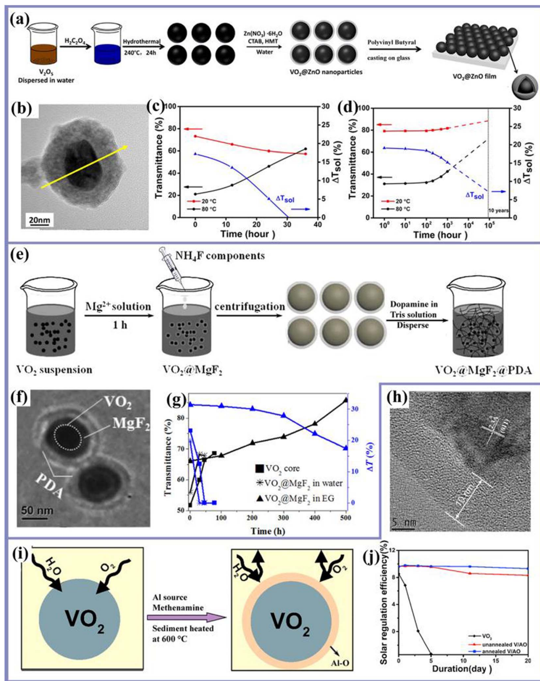
Fig. 1 (a) Experimental flow chart for the synthesis of \text{VO}_2 @ \text{ZnO} core-shell structure nanoparticles and \text{VO}_2 @ \text{ZnO} films. (b) TEM images of \text{VO}_2 @ \text{ZnO} core-shell structure nanoparticles. Optical transmittance spectra of (c) uncoated \text{VO}_2 and (d) \text{VO}_2 @ \text{ZnO} . Reproduced with permission 66 copyright © 2017, American Chemical Society. (e) Flow chart for the whole process of flexible film preparation and influence of reaction parameters for depositing \text{MgF}_2 on the surface of the \text{VO}_2 core. (f) TEM images of \text{VO}_2 nanoparticles with different shell thicknesses of \text{VO}_2 @ \text{MgF}_2 . Vis-IR transmittance spectra of the \text{VO}_2 core. (g) Curves of visible light transmittance and the transmittance difference ( \Delta T ) between room and high temperature at \lambda = 1200 nm of these samples with the change of treatment time. Reproduced with permission 67 Copyright © 2019, American Chemical Society. (h) SEM image of the sample. (i) Preparation of \text{VO}_2 and \text{AlO} . (j) Transmittance spectra with different time spans. Reproduced with permission 69 Copyright © 2017, Elsevier.
