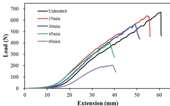
Fig. 5 Tensile strength and strain of the polyester-conductive knitted fabric according to the alkaline hydrolysis duration.
