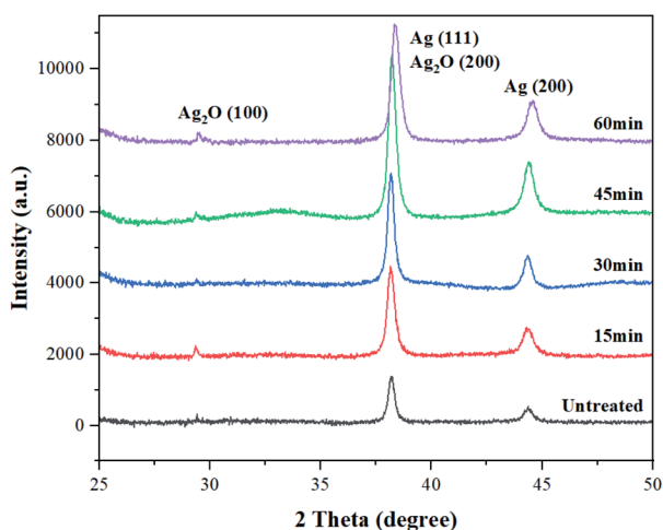
Fig. 6 XRD spectra of conductive yarns according to the alkaline hydrolysis duration.
