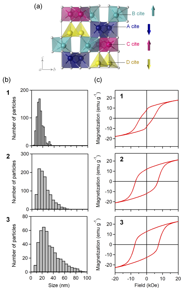
Fig. 1 (a) Crystal structure of \epsilon -Ga x Fe 2-x O 3 . Arrows indicate the sublattice magnetization directions of \epsilon -Ga x Fe 2-x O 3 . (b) The distribution of particle size measured from the TEM images. (c) Magnetic hysteresis loops measured at 300 K.
