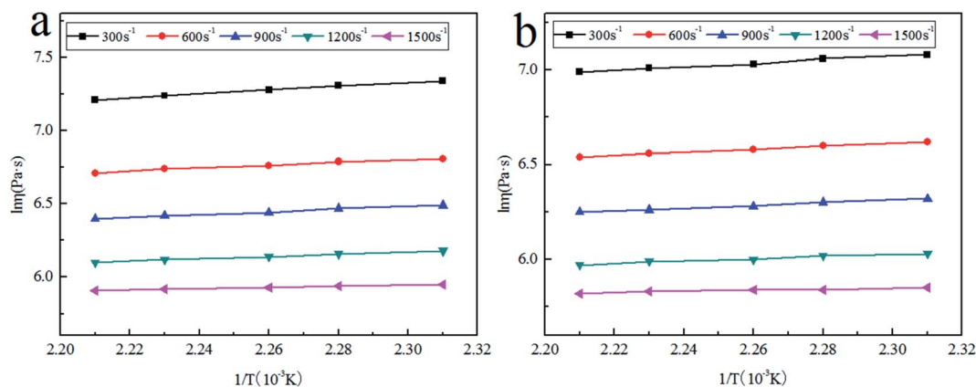
Fig. 8 The logarithm of apparent viscosity ( \ln \eta ) versus 1/T (a) pure LLDPE, (b) LLDPE/P6-0.5% at different shear rates.
