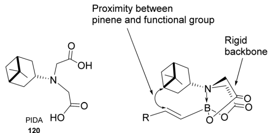
Fig. 11 Pinene-derived iminodiacyclic acid (PIDA).
