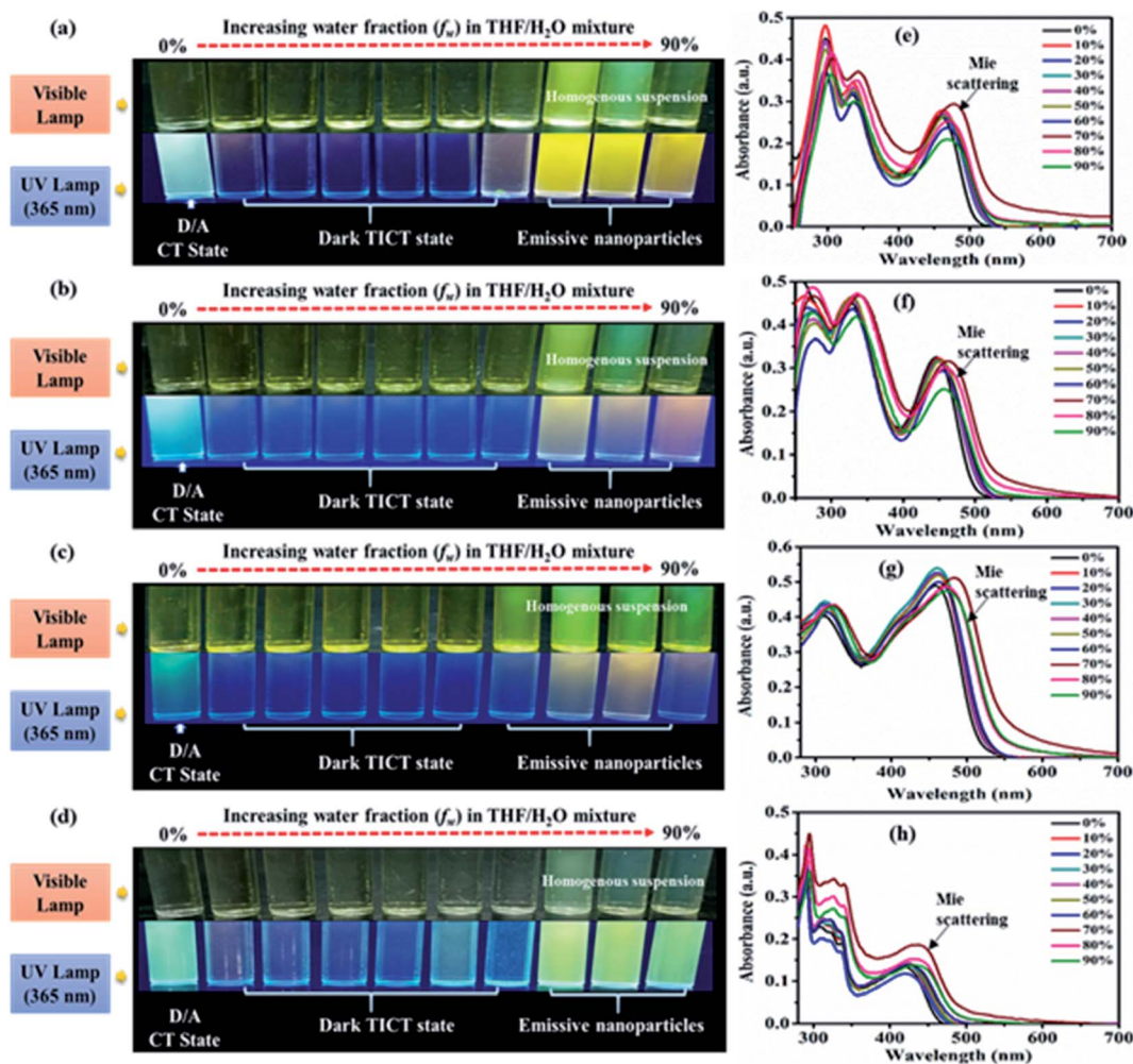
Fig. 7 Emission images of 2 (a), 3 (b), 5 (c) and 7 (d) and absorption spectra of 2 (e), 3 (f), 5 (g) and 7 (h) recorded in 10 \mu\text{M} solution of different THF-H 2 O mixtures with increasing percentage of water fraction ( f_w ).
