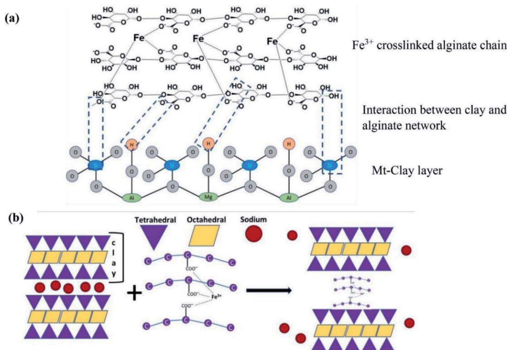
Fig. 4 (a) The crosslinking process of \text{Fe}^{3+} to Alg network and interaction with Mt and (b) the possible MtAlg network configuration. This figure reproduced from ref. 82 with permission from Elsevier. Copyright (2021).
