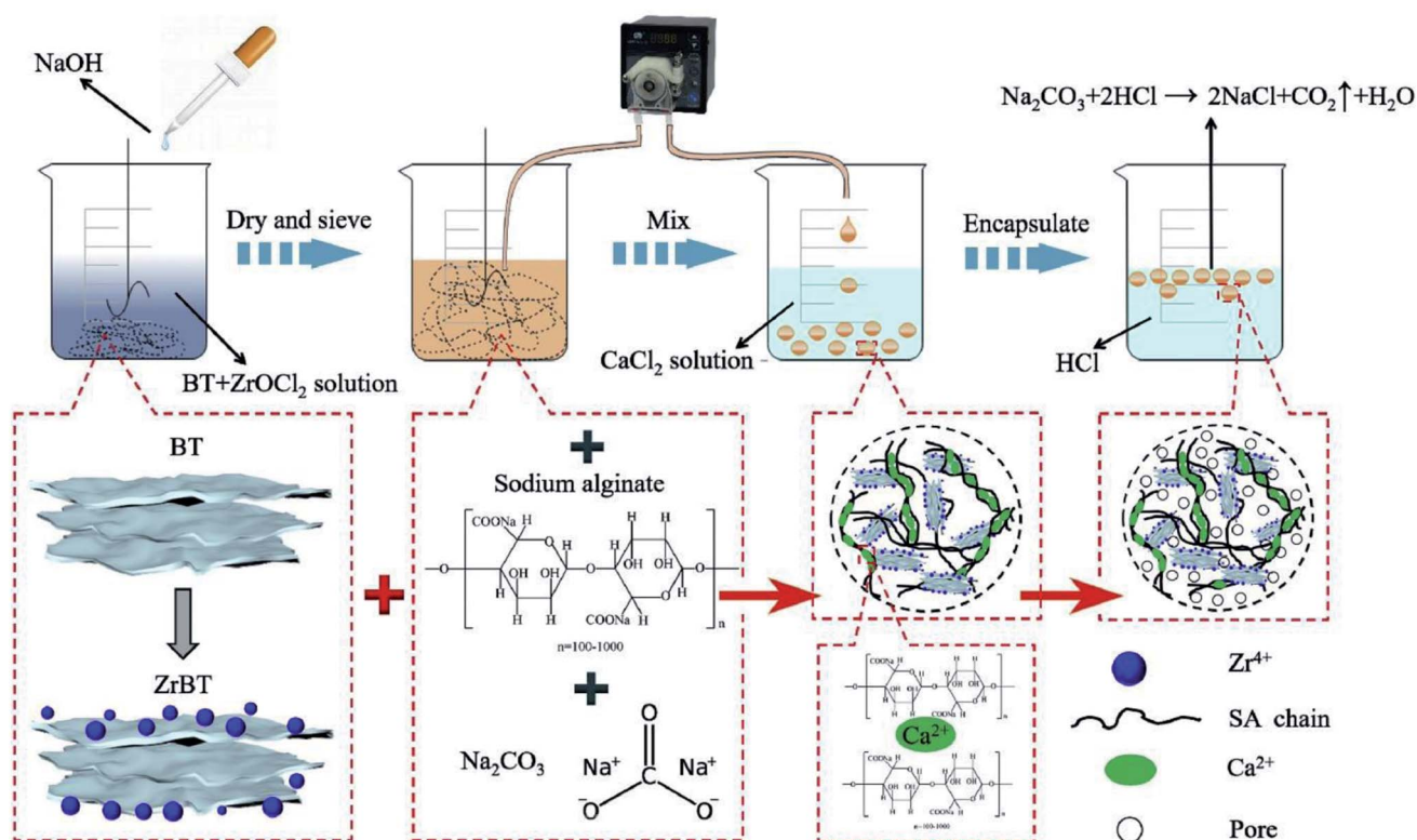
Fig. 8 Illustration of the fabrication process of NH-Alg-ZrBT. This figure reproduced from ref. 93 with permission from Elsevier. Copyright (2021).
