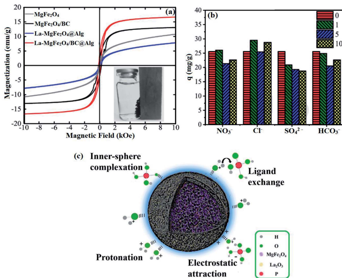
Fig. 9 (a) VSM measurement, (b) effect of different concentrations of coexisting ions on phosphate adsorption, and (c) the proposed adsorption mechanisms of phosphate onto La- \text{MgFe}_2\text{O}_4/\text{BC}@\text{Alg} . This figure reproduced from ref. 100 with permission from Elsevier. Copyright (2021).
