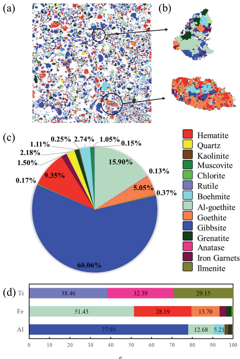
Fig. 3 The AMICS results for gibbsitic bauxite (a) and (b) minerals distribution, (c) minerals proportions, and (d) proportions of Ti, Fe, Al in minerals.
