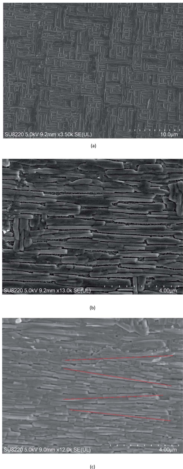
Fig. 2 Typical SEM images of K_{0.3}MoO_3 thin films grown (a) on SrTiO_3(100) , (b) on SrTiO_3(510) , (c) on SrTiO_3(110) , respectively. The red line on SrTiO_3(110) suggest the multidirectional growth of grains comparing with the unidirectional growth of grains on SrTiO_3(510) .
