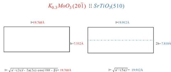
Fig. 3 Schematic of the lattice match leading to K_{0.3}MoO_3(201) and SrTiO_3(510) . The length of the K_{0.3}MoO_3(201) lattice plane is calculated by cosine rule and the length of SrTiO_3(510) is calculated by Pythagorean theorem.
