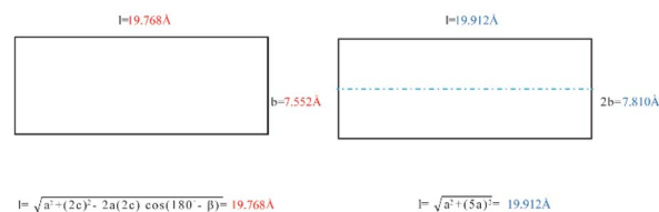
Fig. 3 Schematic of the lattice match leading to K_{0.3}MoO_3(201) and SrTiO_3(510) . The length of the K_{0.3}MoO_3(201) lattice plane is calculated by cosine rule and the length of SrTiO_3(510) is calculated by Pythagorean theorem.
