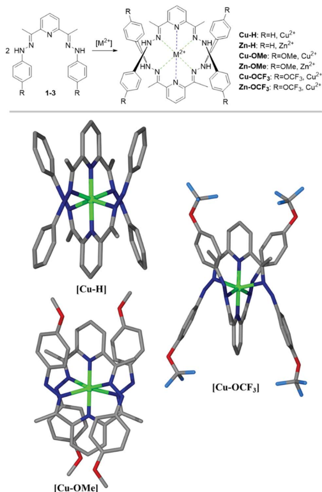
Fig. 5 Formation of the metal complexes showing the axial Py-metal bonds (blue) and the equatorial imino-metal bonds (green). Crystal structures of Cu(II) complexes determined by X-ray analysis. Pictures are presented with non-hydrogen atoms displayed.
