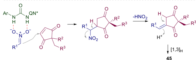
Scheme 33 Alkylation of cyclopentenedione derivatives catalyzed by quinine-derived chiral urea 44 .
