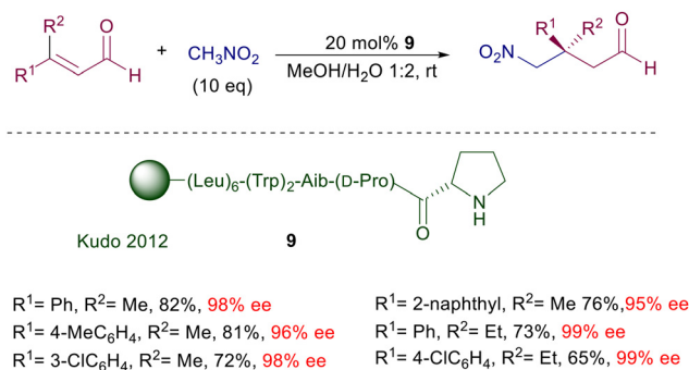
Scheme 6 Resin-bound peptide catalyst bearing a terminal proline residue.
