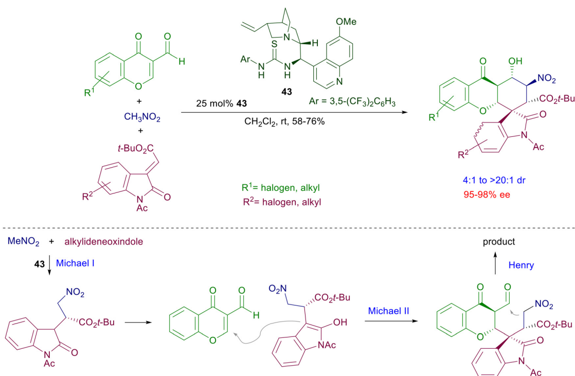
Scheme 32 Three-component cascade process catalyzed by chiral thiourea 43 leading to spiroindole derivatives.
