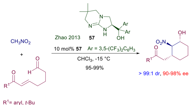
Scheme 41 Chiral bicyclic guanidine 57 as catalyst for the tandem conjugate addition/aldol condensation of nitromethane to oxoals.
