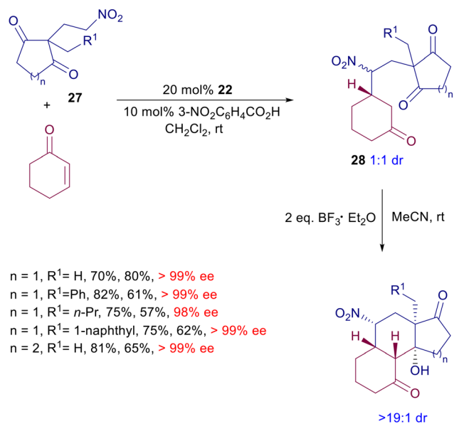
Scheme 21 Synthesis of cis,cis -tricyclic diterpenoid derivatives by a tandem conjugate addition/aldol condensation catalyzed by quinine-derived amine 22 .
