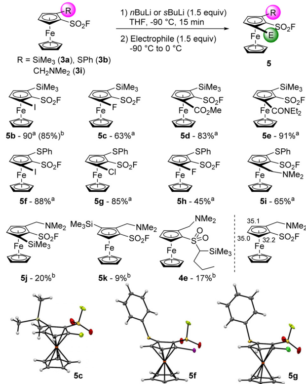
Scheme 3 Deprotolithiation-electrophilic trapping sequence from the 1,2-disubstituted ferrocenes 3 . a Reaction performed with s BuLi. b Reaction performed with n BuLi.
