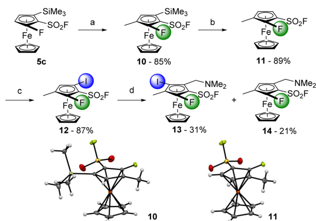
Scheme 7 Deprotolithiation-electrophilic trapping sequence towards the 1,2,3,4,5-pentasubstituted ferrocene 13 . Reaction conditions: (a) (i) \text{sBuLi} (1.2 equiv.), THF, -80^\circ\text{C} , 1 h; (ii) \text{CH}_3\text{I} (1.2 equiv.), -80^\circ\text{C} to rt; (b) TBAF (1.5 equiv.), THF, 0^\circ\text{C} , 5 min; (c) (i) \text{sBuLi} (1.5 equiv.), THF, -90^\circ\text{C} , 1 h; (ii) \text{I}_2 (1.2 equiv.), -80^\circ\text{C} to rt; (d) (i) LiTMP (1.1 equiv.), THF, -50^\circ\text{C} , 1 h; (ii) \text{H}_2\text{C}=\text{NMe}_2 (1.1 equiv.), -50^\circ\text{C} to rt.
