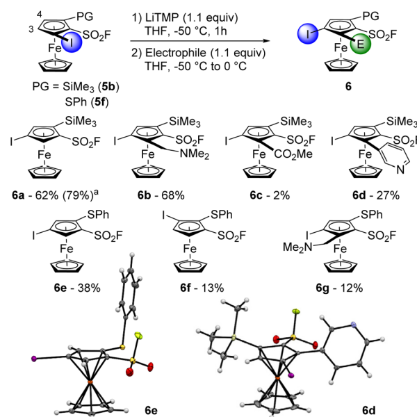
Scheme 5 Deprotection-lithiation-electrophilic trapping sequence from the 1,2-disubstituted ferrocenes 5b and 5f . a Reaction performed on a 16 mmol scale.
