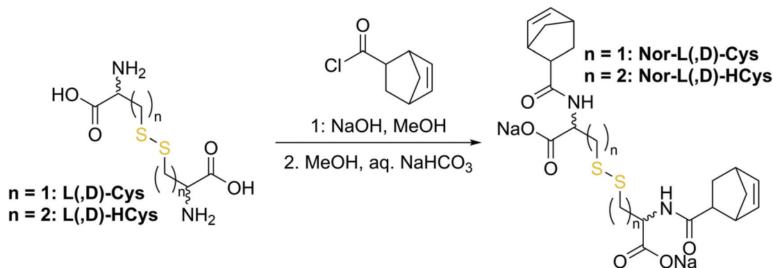
Scheme 2 Synthesis of cysteine- and homocysteine-based linkers.
