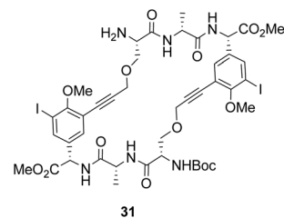
Fig. 12 By-product cyclic dimer 31 .
