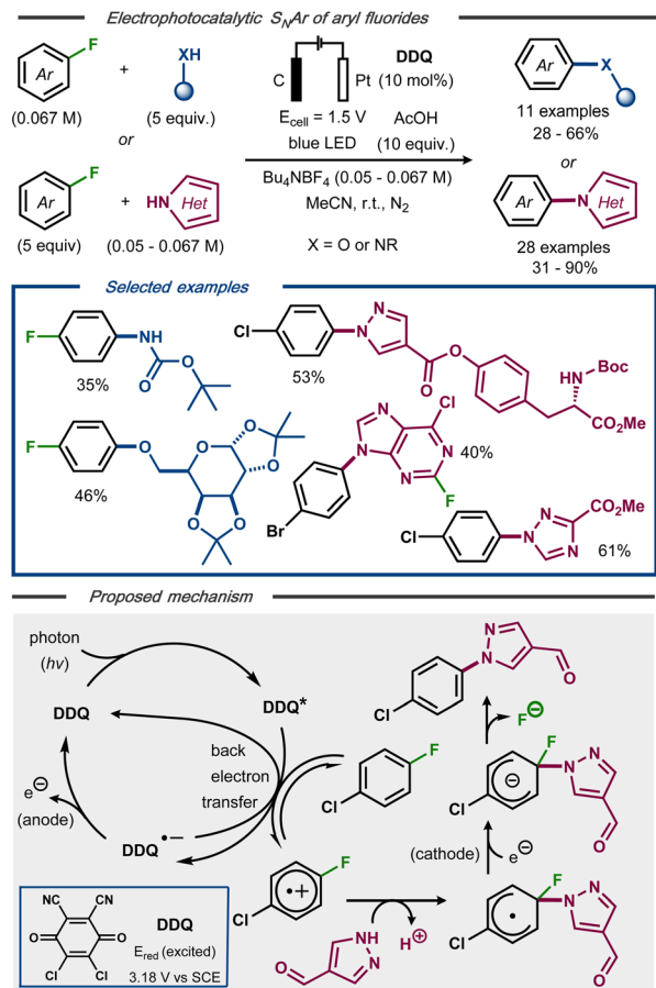
Fig. 9 Top: Electrophotochemical nucleophilic aromatic substitution of aryl fluorides. 46 Bottom: Proposed mechanism.
