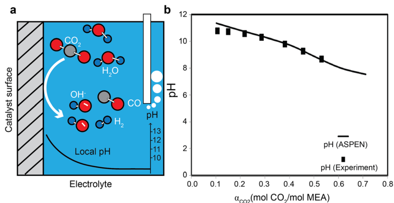
Fig. 4 (a) A schematic illustration of local pH difference for gas-fed \text{CO}_2 electroreduction close to the catalyst surface. (b) The pH evolution as a function of \text{CO}_2 loading in 30 wt% MEA aqueous solution at 21 °C. Reproduced with permission, 54 copyright 2012, American Chemical Society.
