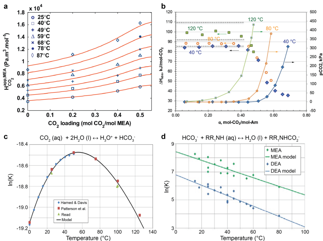
Fig. 3 The temperature effects on (a) Henry constant of \text{CO}_2 , reproduced with permission, 49 copyright 2011, Elsevier. (b) \text{CO}_2 partial pressure and heat of \text{CO}_2 absorption for 30 wt% MEA aqueous solutions, reproduced with permission, 50 copyright 2014, Elsevier, (c) bicarbonate formation, and (d) carbamate formation for MEA and DEA aqueous solution. Reproduced with permission, 51 copyright 2017, Elsevier.
