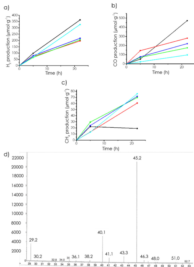
Fig. 3 Temporal gas evolution from CO _2 dissolved in a CH _3 CN/H _2 O mixture containing TEAO using mp-C \alpha (black), mp-C \beta (red), mp-C \gamma (green), mp-(N)-C \alpha (blue), and mp-(P)-C \alpha (cyan) as photocatalysts upon 300 W Xe lamp irradiation: (a) H _2 , (b) CO, (c) CH _4 , (d) mass spectra of the test using ^{13} CO _2 as the substrate and mp-C \alpha as the photocatalyst.
