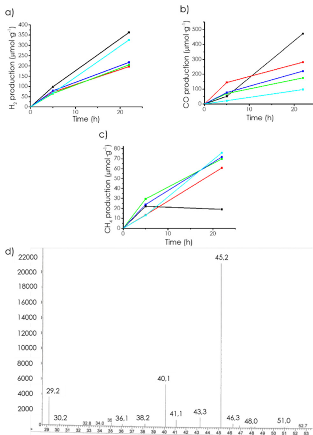
Fig. 3 Temporal gas evolution from CO _2 dissolved in a CH _3 CN/H _2 O mixture containing TEOA using mp-C _{\alpha} (black), mp-C _{\beta} (red), mp-C _{\gamma} (green), mp-(N)-C _{\alpha} (blue), and mp-(P)-C _{\alpha} (cyan) as photocatalysts upon 300 W Xe lamp irradiation: (a) H _2 , (b) CO, (c) CH _4 , (d) mass spectra of the test using ^{13} CO _2 as the substrate and mp-C _{\alpha} as the photocatalyst.
