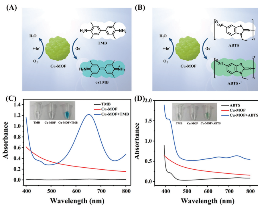
Fig. 4 Schematic illustration of the oxidase-like activity of Cu-MOFs for TMB (A) and ABTS (B). The UV-vis spectra of TMB (C) and ABTS (D) in the absence and presence of Cu-MOFs. Inserts: the color change of the corresponding solution.
