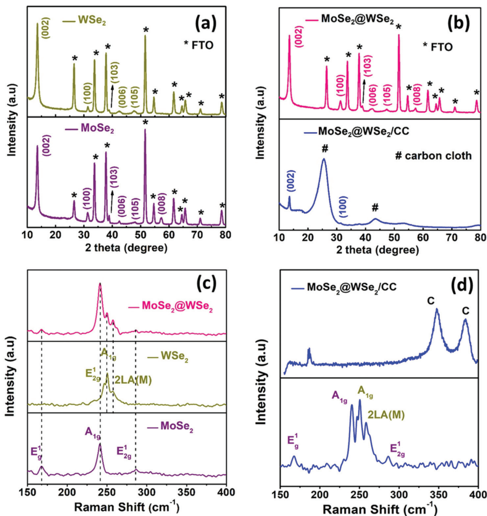
Fig. 3 XRD pattern (a) \text{WSe}_2 and \text{MoSe}_2 (b) \text{MoSe}_2@\text{WSe}_2/\text{FTO} and \text{MoSe}_2@\text{WSe}_2/\text{CC} . Raman spectra (c) \text{WSe}_2 and \text{MoSe}_2 (d) \text{MoSe}_2@\text{WSe}_2/\text{FTO} and \text{MoSe}_2@\text{WSe}_2/\text{CC} .
