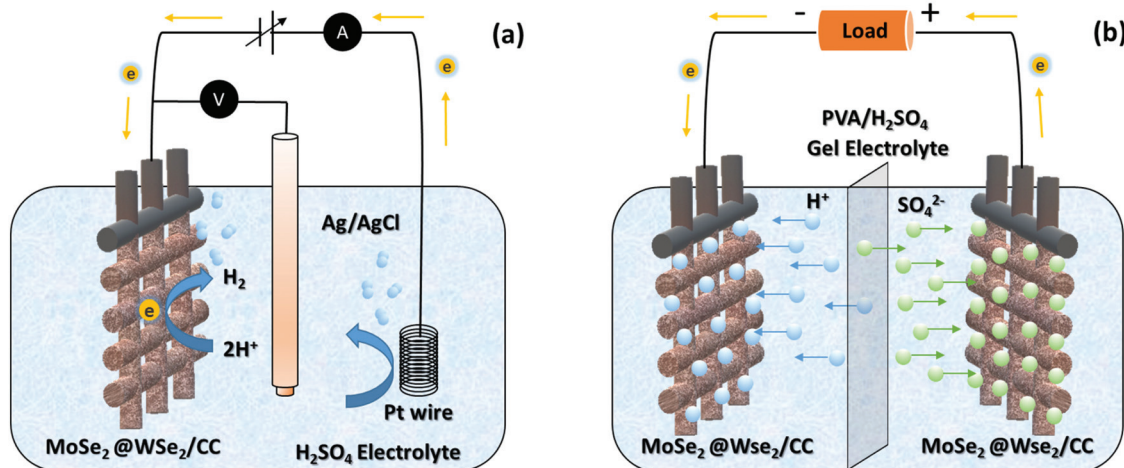
Fig. 8 The schematic working mechanism of (a) hydrogen evolution and (b) FSSC-based on MoSe 2 @WSe 2 HS composite on CC.
